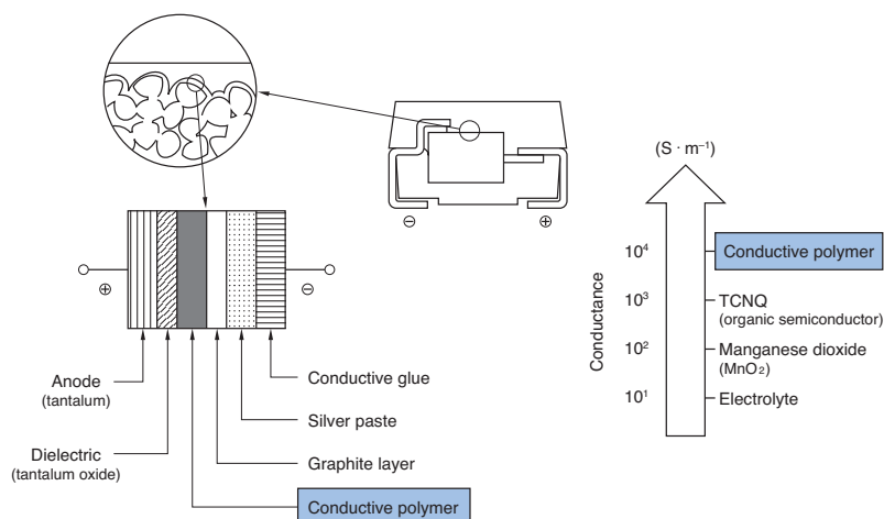
NeoCapacitor's Structure
